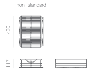
1 Layer Injection Drawer / D1-SIS-400 400 Compatible
