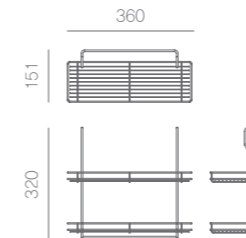
Double layer shelf / D1-A2D
