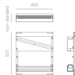
Board type D1-YID-P
