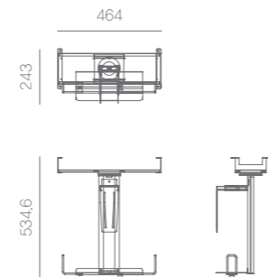
Rotating Type / D3-PCH-3
