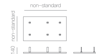
Magnetic Mat / D1-SMM-600 600 Compatible (Non-standard Production Available)
