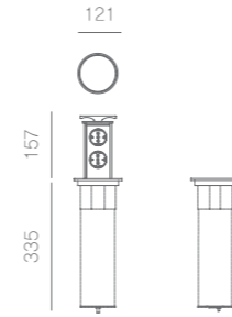
D1-CJA-C2 / 2 Sockets Size of die cutting on top board: 105mm
